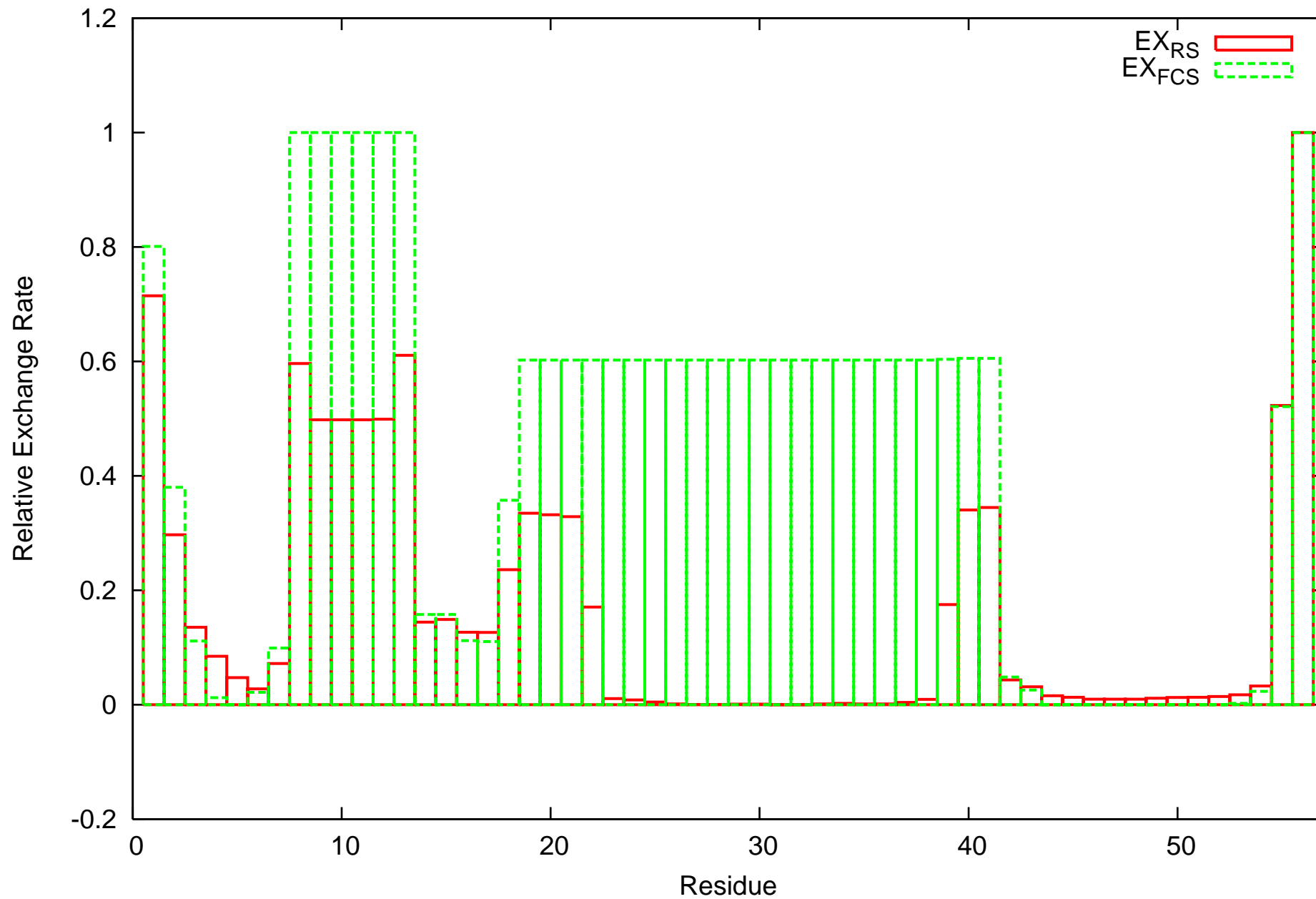
Relative Hydrogen Exchange Rates: 1GB1, Map R714-1GB1
