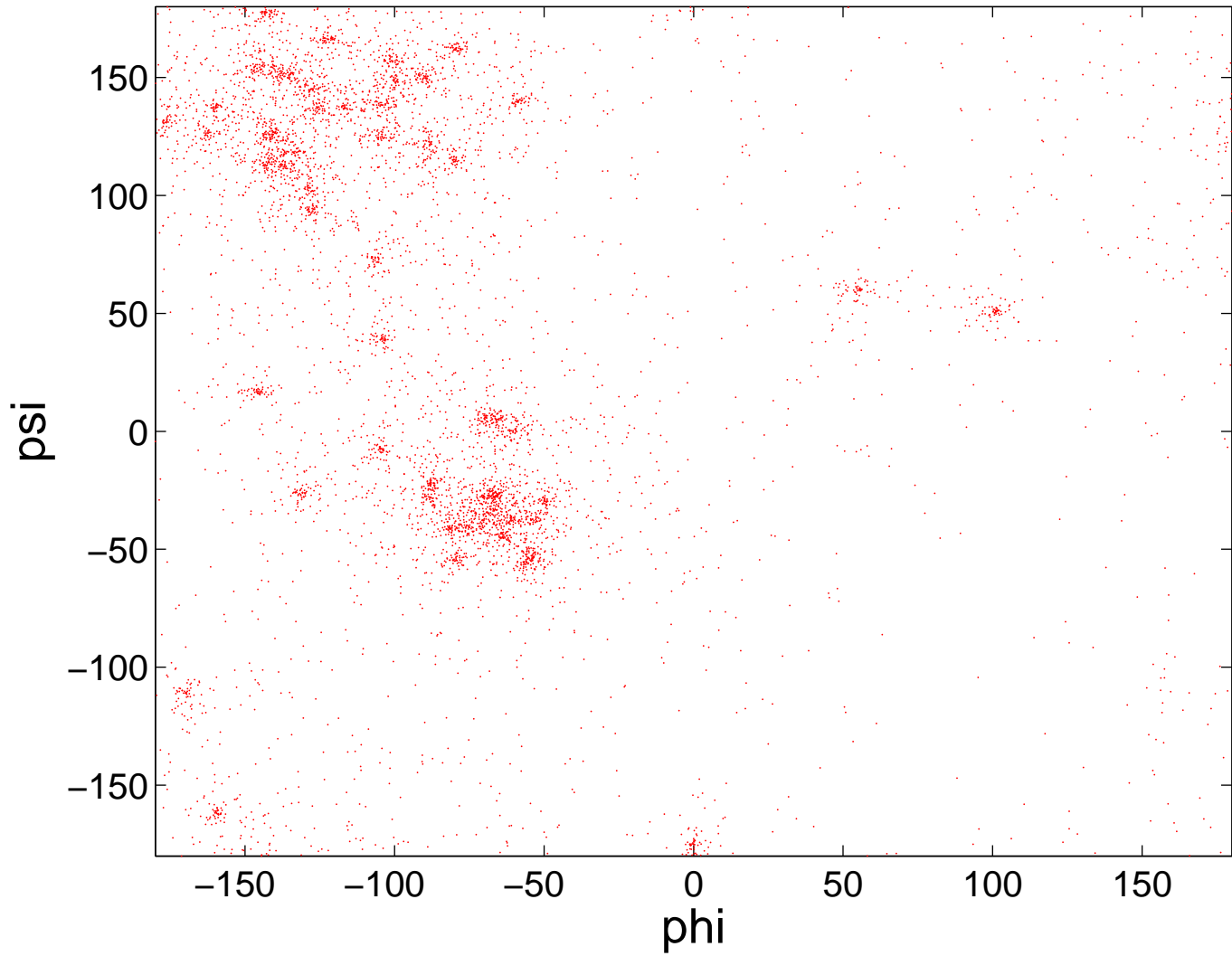
Ramachandran Plot: 1GB1, Map R714-1GB1
