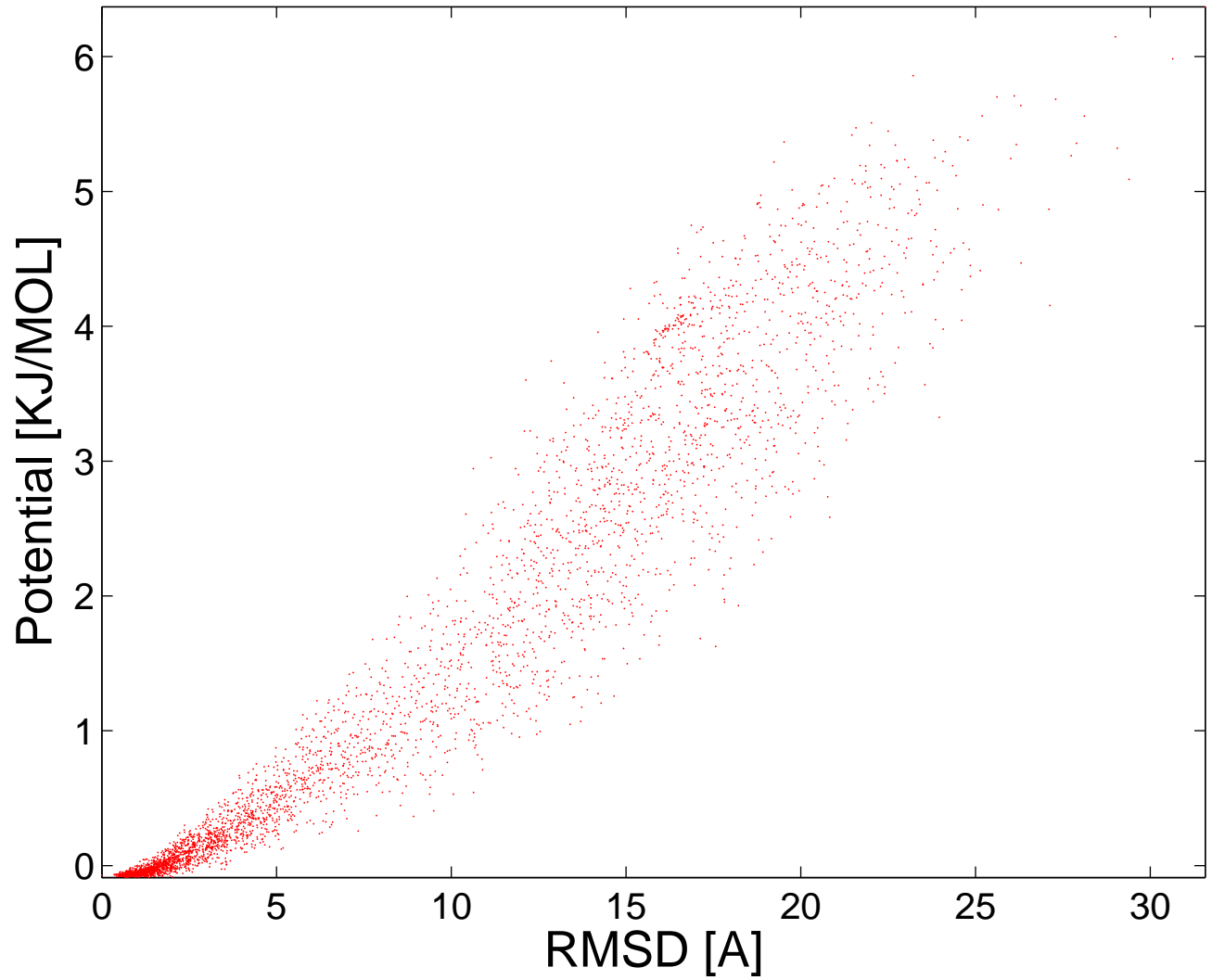
Potential vs. RMSD: 1GB1, Map R714-1GB1
