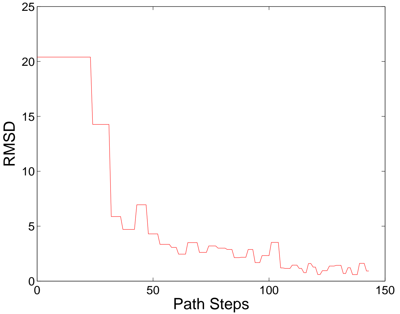
RMSD Profile: 1GB1, Path R714-1GB1.SSFO80-0
