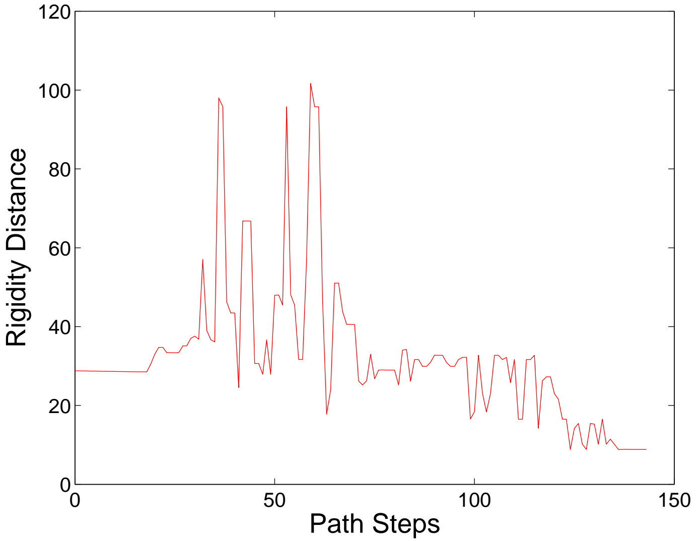
Rigidity Distance Profile: 1GB1, Path R714-1GB1.SSFO80-0
