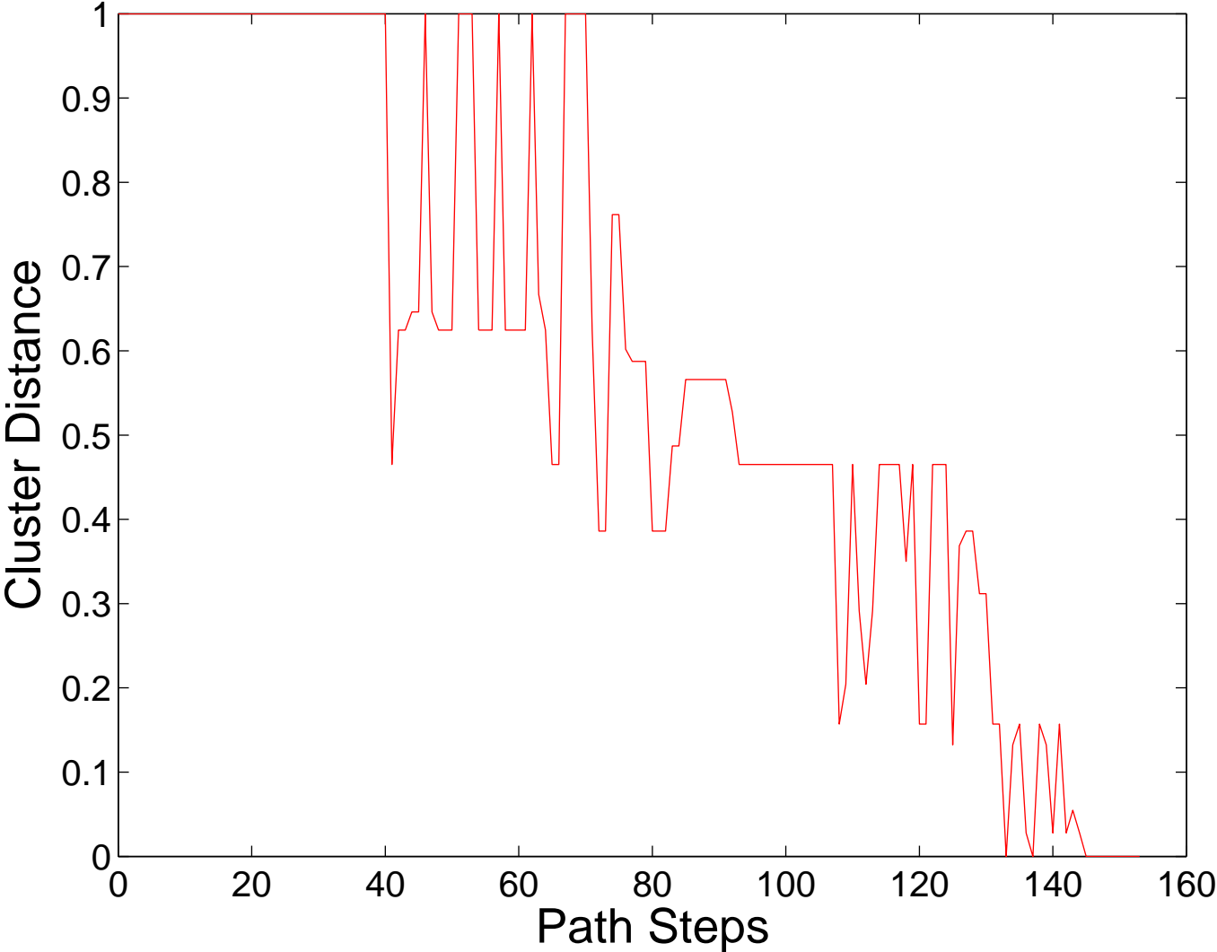
Cluster Distance Profile: 1GB1, Path R714-1GB1.SSFO80-1
