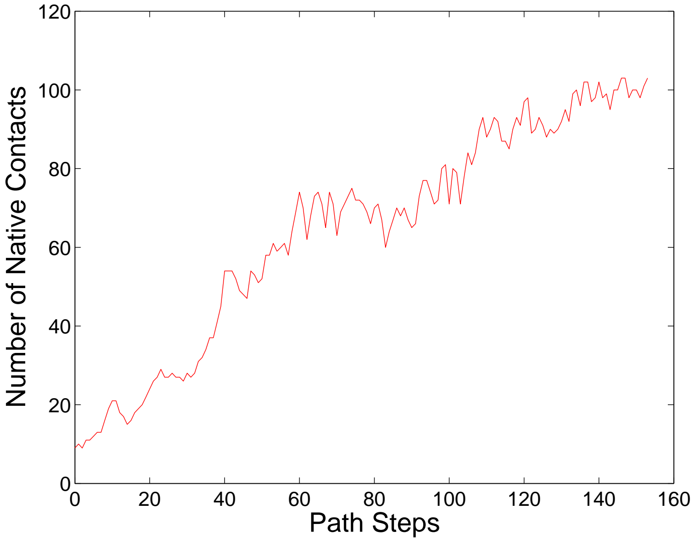
All Contact Profile: 1GB1, Path R714-1GB1.SSFO80-1
