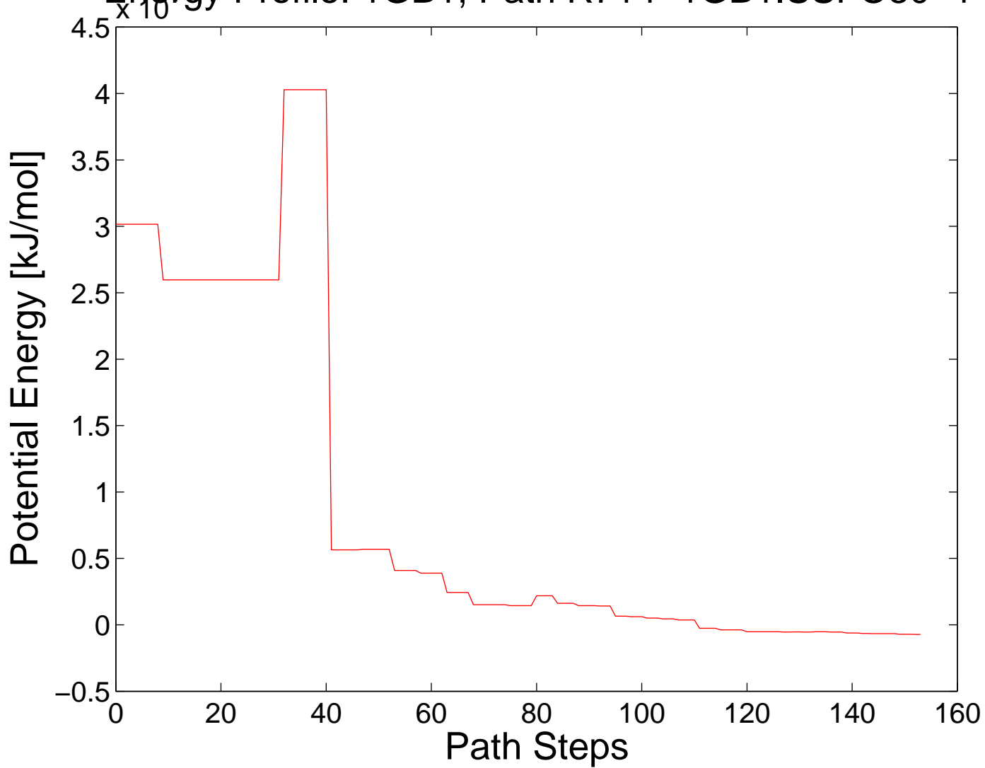
Energy Profile: 1GB1, Path R714-1GB1.SSFO80-1
