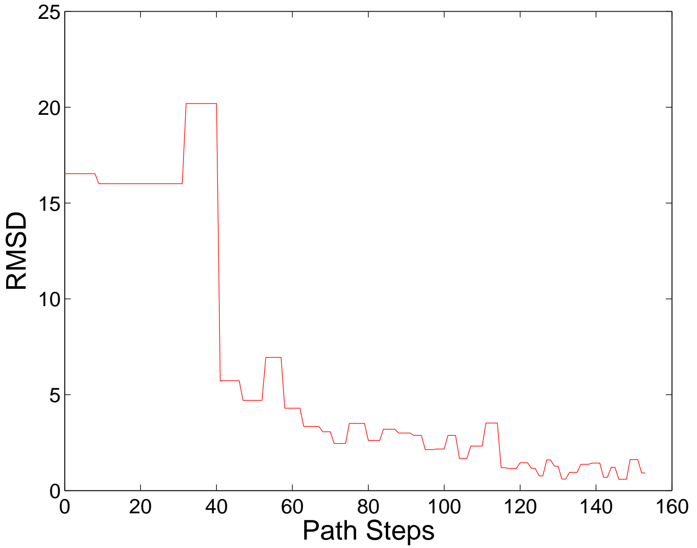
RMSD Profile: 1GB1, Path R714-1GB1.SSFO80-1
