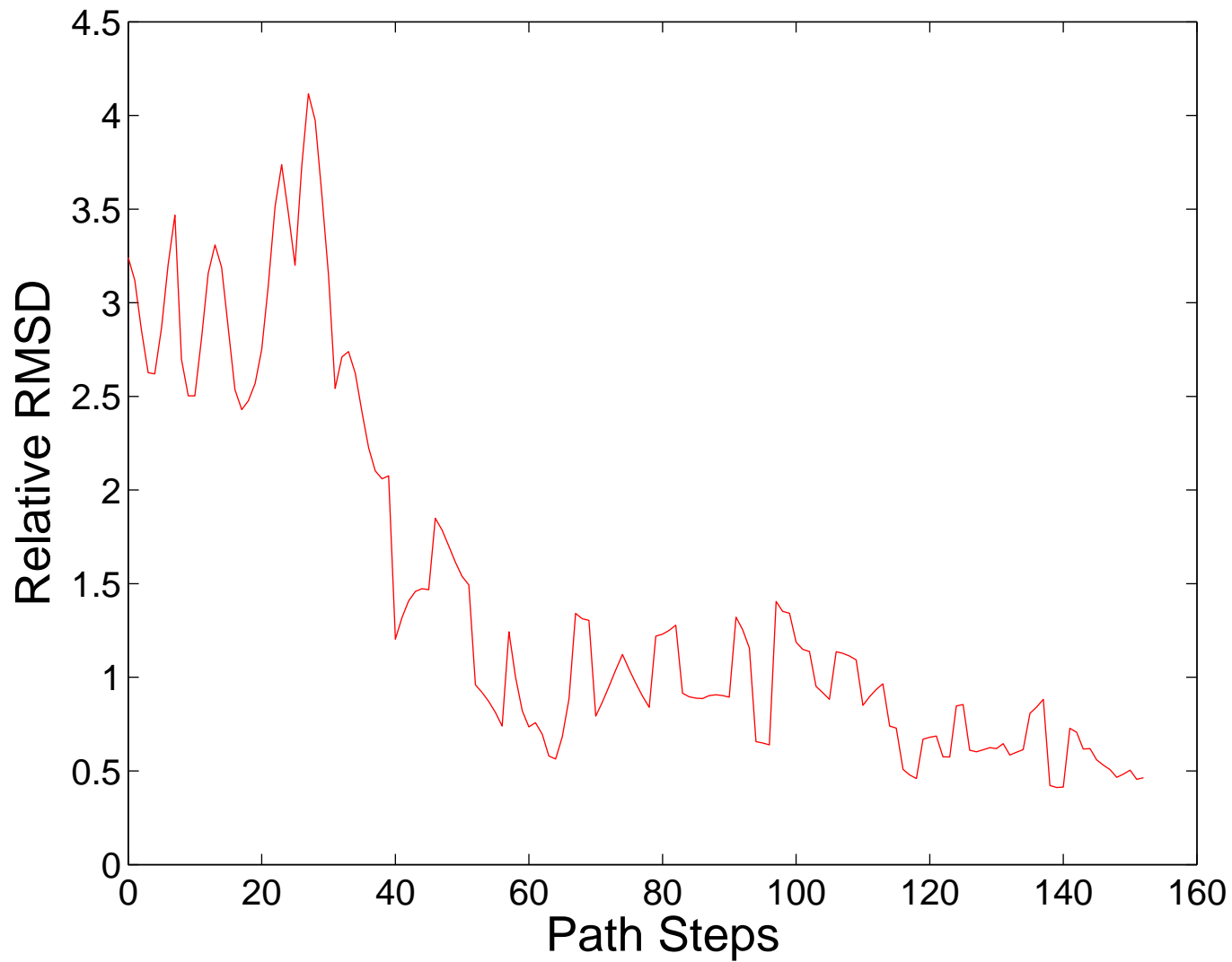
Relative RMSD Distance Profile: 1GB1, Path R714-1GB1.SSFO8C
