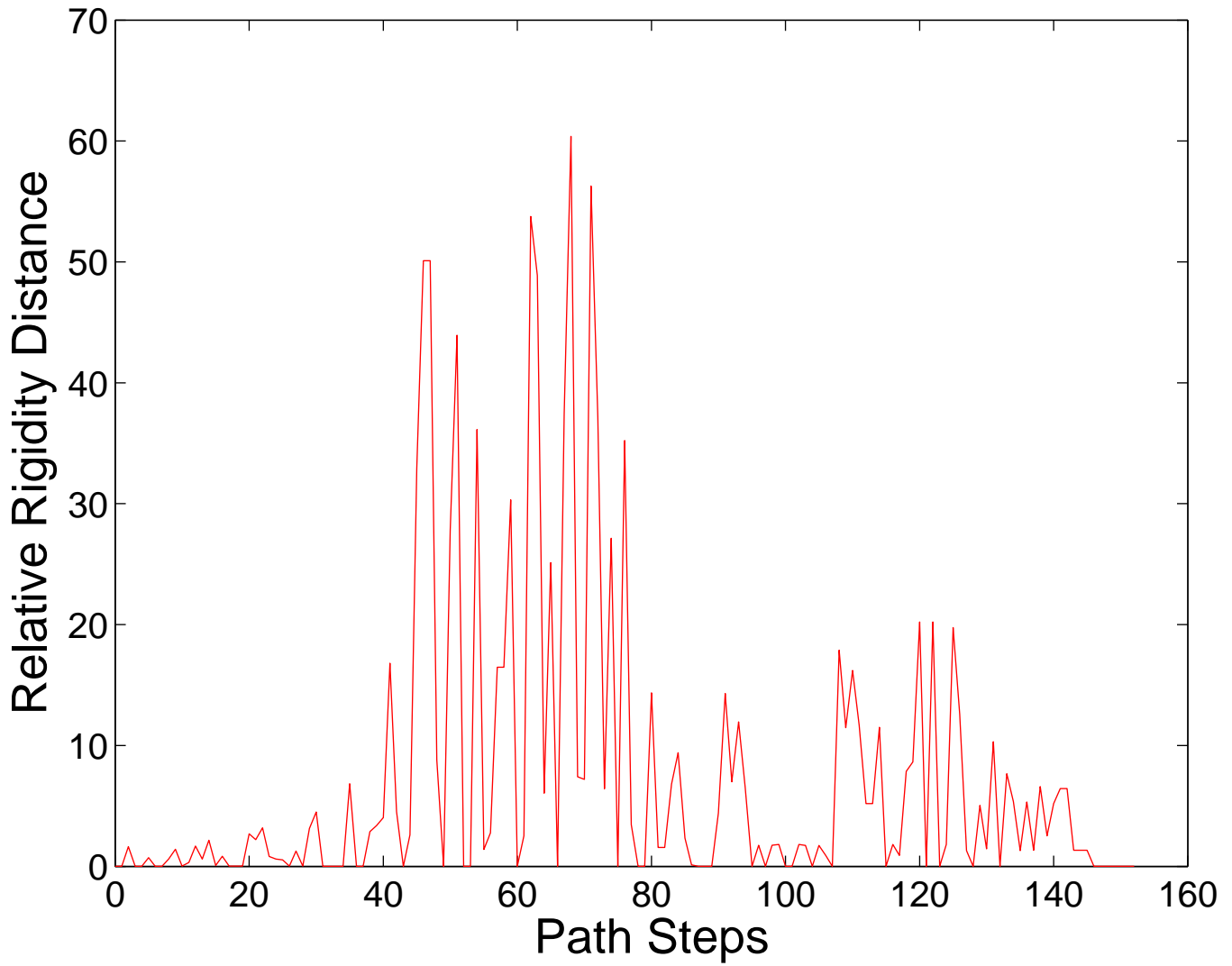
relative Rigidity Distance Profile: 1GB1, Path R714-1GB1.SSFO80
