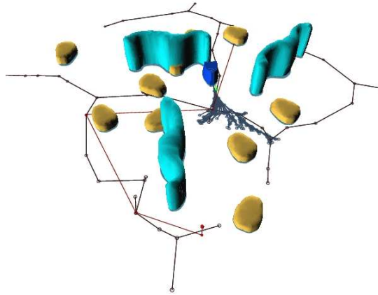
Figure 5: In this environment, the robot must navigate around the spinning rotors trying to avoid soft objects in the environment.
